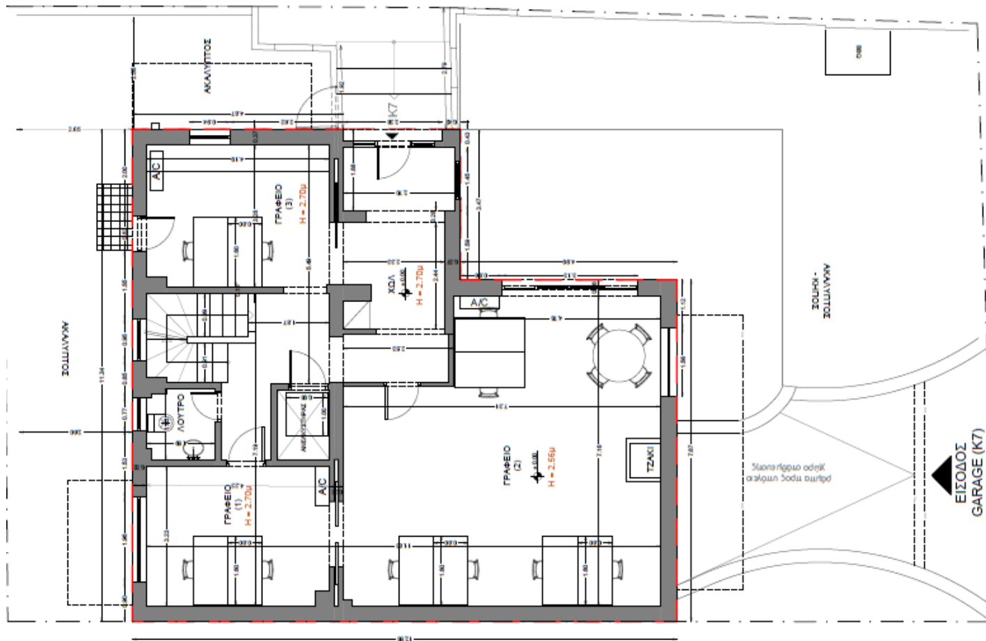
GROUND FLOOR
